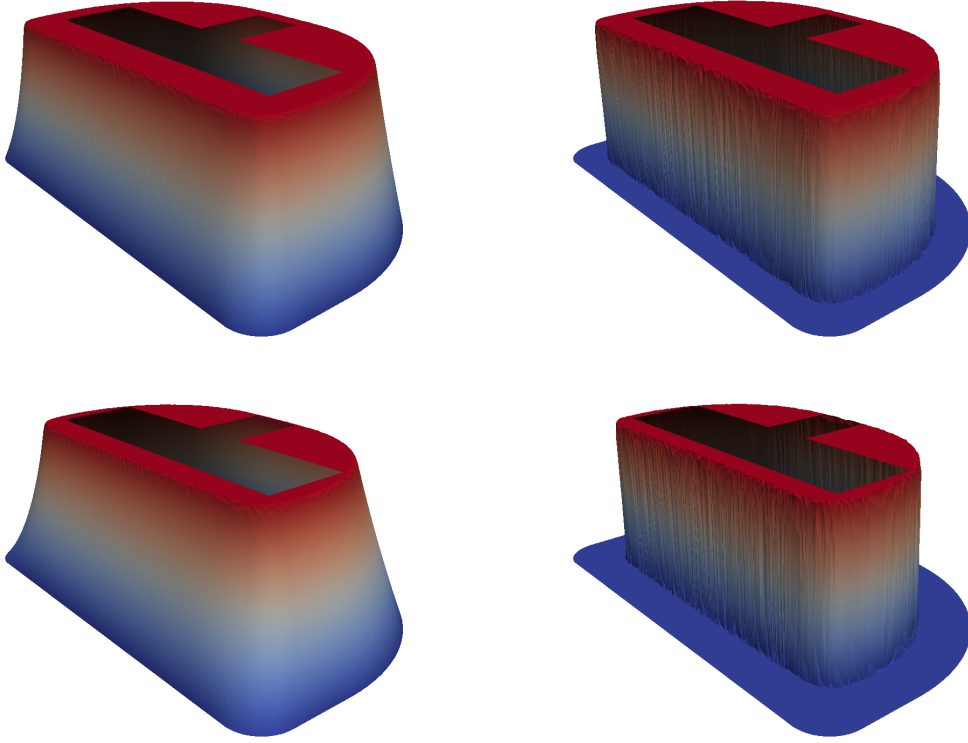
Figure 4: Three-dimensional profile of the dissolved drug concentration C (left) and the area of solid particles per unit volume a (right) for t = 84hs (top) and t = 168hs (bottom). We see that C \approx C_s where a > 0 and C looks like a solution to a pure diffusion equation where a = 0 , with a Robin-type boundary condition in the outer boundary.
